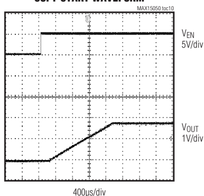
SOFT-START WAVEFORM
